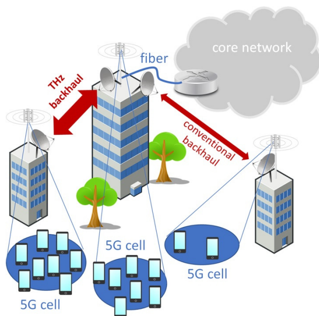
Figure: Application of THz backhaul links in future cellular networks Picture credits: TU Braunschweig
